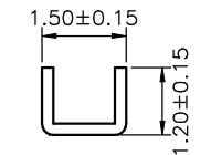
SEC:C-C
